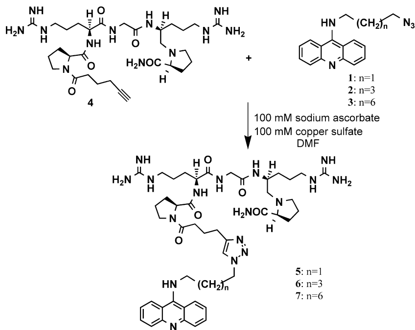
Scheme 2. Synthesis of authentic sample for adducts between peptide and acridine derivatives.
